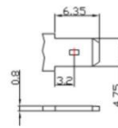
F2 Terminal (Brass Coated with Silver)
